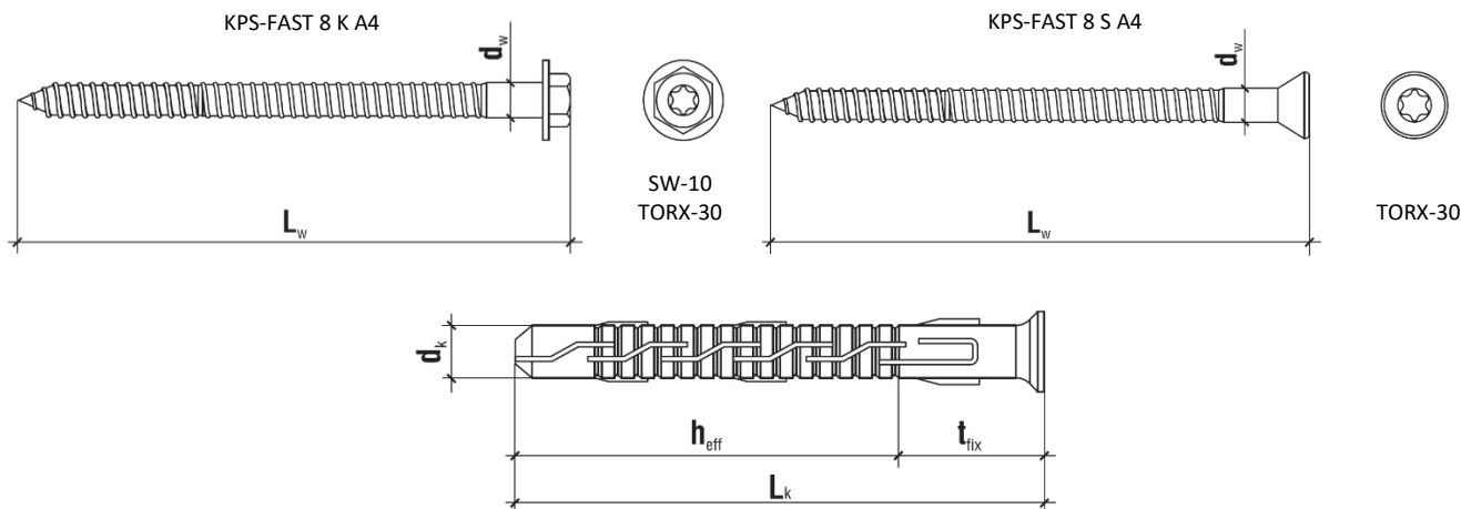
SELECTION TABLE – KPS-FAST 8 K A4
